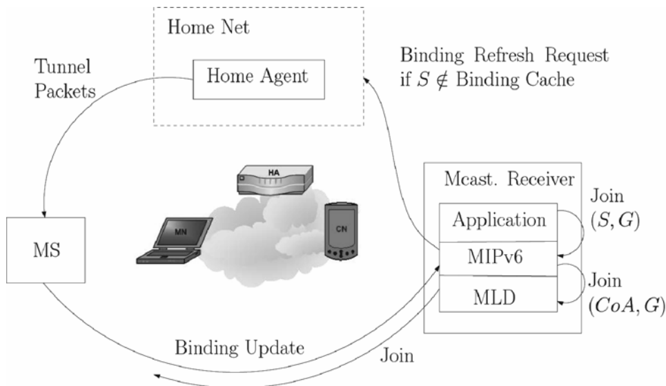
Fig. 1. Initial care-of address discovery by receiver’s mobile IPv6 stack
